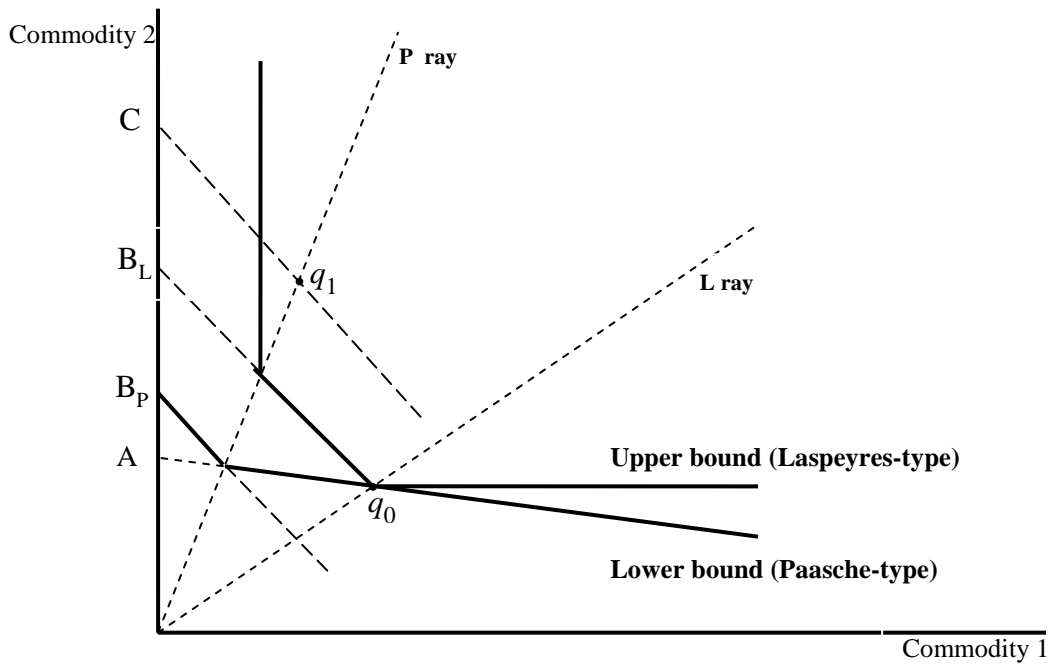
Figure 2: Laspeyres- and Paasche-type bounds based on q_0
