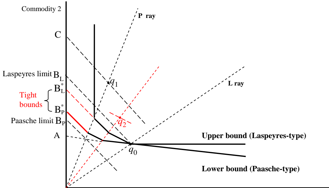
Figure 4: Tightening the bounds by adding a third observation point
