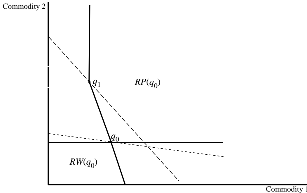
Figure 1: RP(q_0) and RW(q_0) : simple case of “revealed preference test.”
